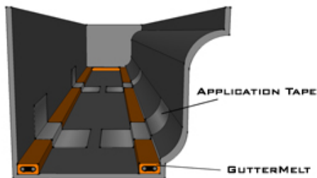
GUTTER CROSS SECTION
